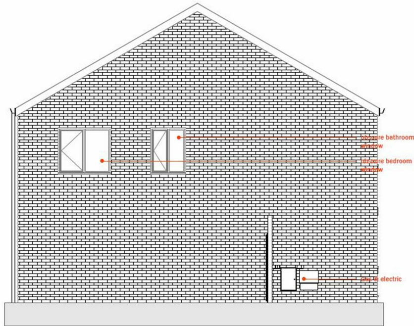
1 Proposed West Elevation SCALE: 1:50
