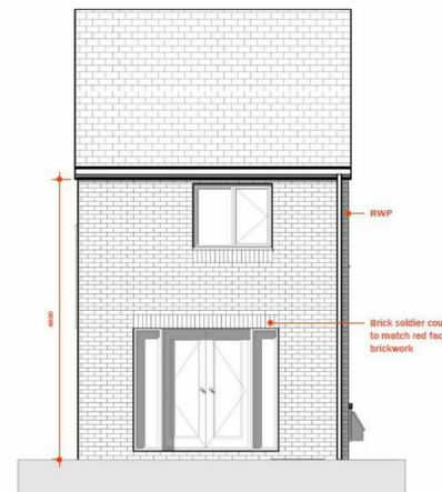
2 Proposed Rear Elevation
